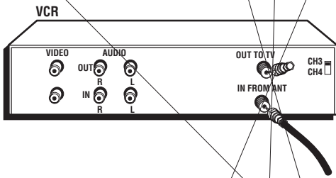
From Cable or Antenna
